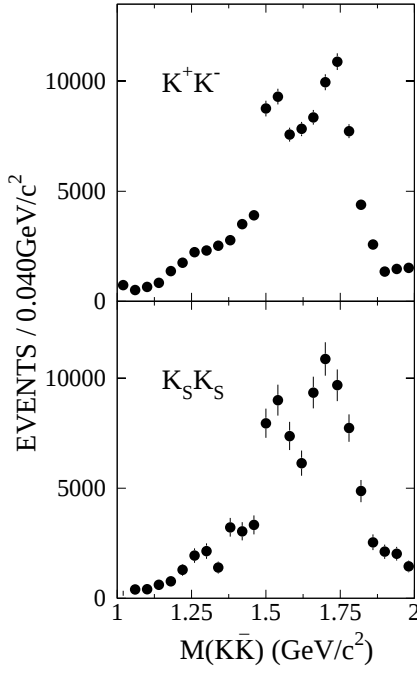
FIG. 2. The K\bar{K} mass distributions from J/\psi radiative decays to K^+K^- (upper) and K_S^0K_S^0 (lower) after acceptance and isospin corrections.
