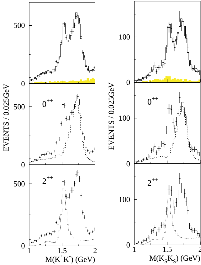
FIG. 4. The K\bar{K} invariant mass distributions from J/\psi \rightarrow \gamma K^+ K^- and J/\psi \rightarrow \gamma K_S^0 \bar{K}_S^0 . The points are the data and the full histograms in the top panels show the maximum likelihood fit. Histograms on subsequent panels show the complete 0^+ and 2^+ contributions including all interferences.
