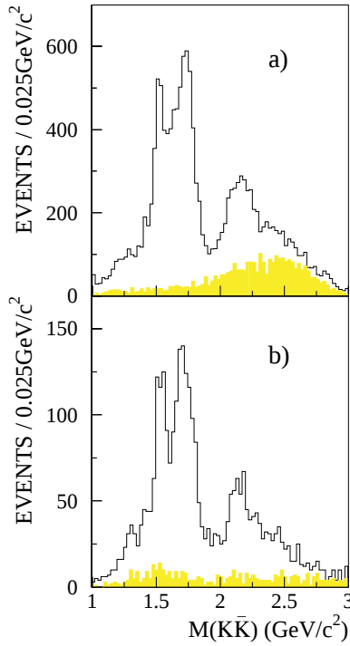
FIG. 1. Invariant mass spectra of (a) K^+ K^- , (b) K_S^0 \bar{K}_S^0 for J/\psi \rightarrow \gamma K \bar{K} events, where the shaded histograms correspond to the estimated background contributions.
